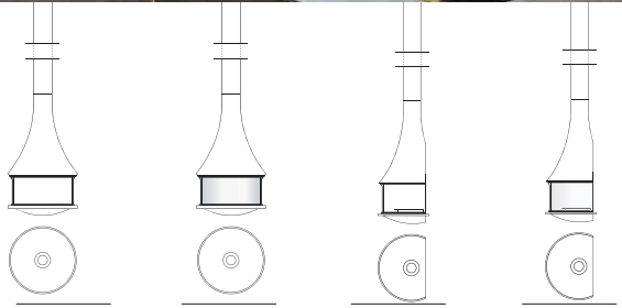
centrale color foyer ouvert central color open fire centrale color vitrée central color with glass enclosure murale color foyer ouvert wall-mounted color open fire murale color vitrée wall-mounted color with glass enclosure DISPONIBLE EN 180 COULEURS RAL | AVAILABLE IN 180 RAL COLORS DISPONIBLE VERNIS INCOLORE ET VERNIS FONCÉ | AVAILABLE CLEAR VARNISH AND DARK VARNISH
