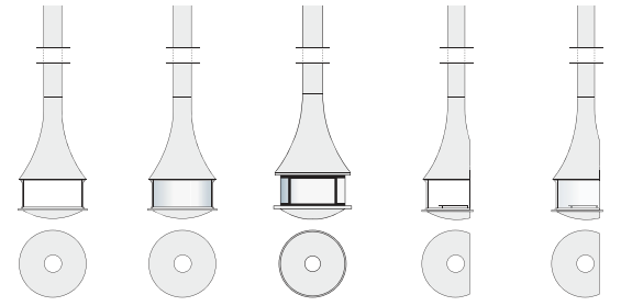
centrale foyer ouvert central open fire centrale vitrée central with glass enclosure centrale vitrée sérigraphiée central with silk-screen printed glass enclosure murale foyer ouvert wall-mounted open fire murale vitrée wall-mounted with glass enclosure
